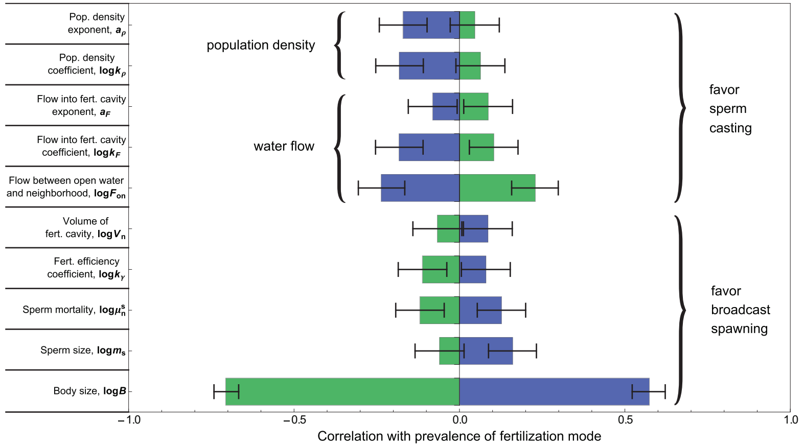
Figure 7: Correlation of selected parameters with the prevalence of stable sperm casting (green) and broadcast spawning (blue) in trials with randomly chosen body size, shown with 99% confidence intervals. Positive correlations indicate that the prevalence of a fertilization mode was associated with larger values of the parameter. Only parameters that were significantly correlated with at least one fertilization mode are shown.
